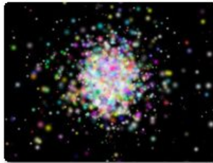
Particles
